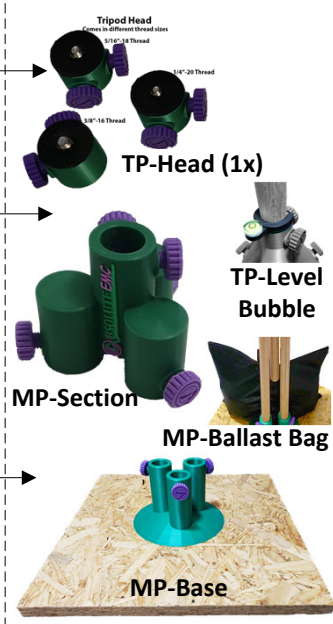
Absolute EMC Monopole
